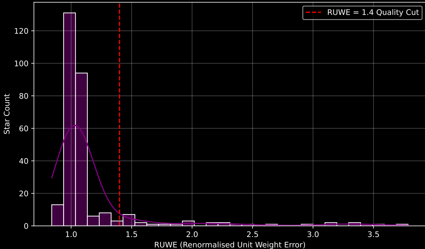
GALAH DR4 Field [1616] RUWE Distribution (n= 285)
