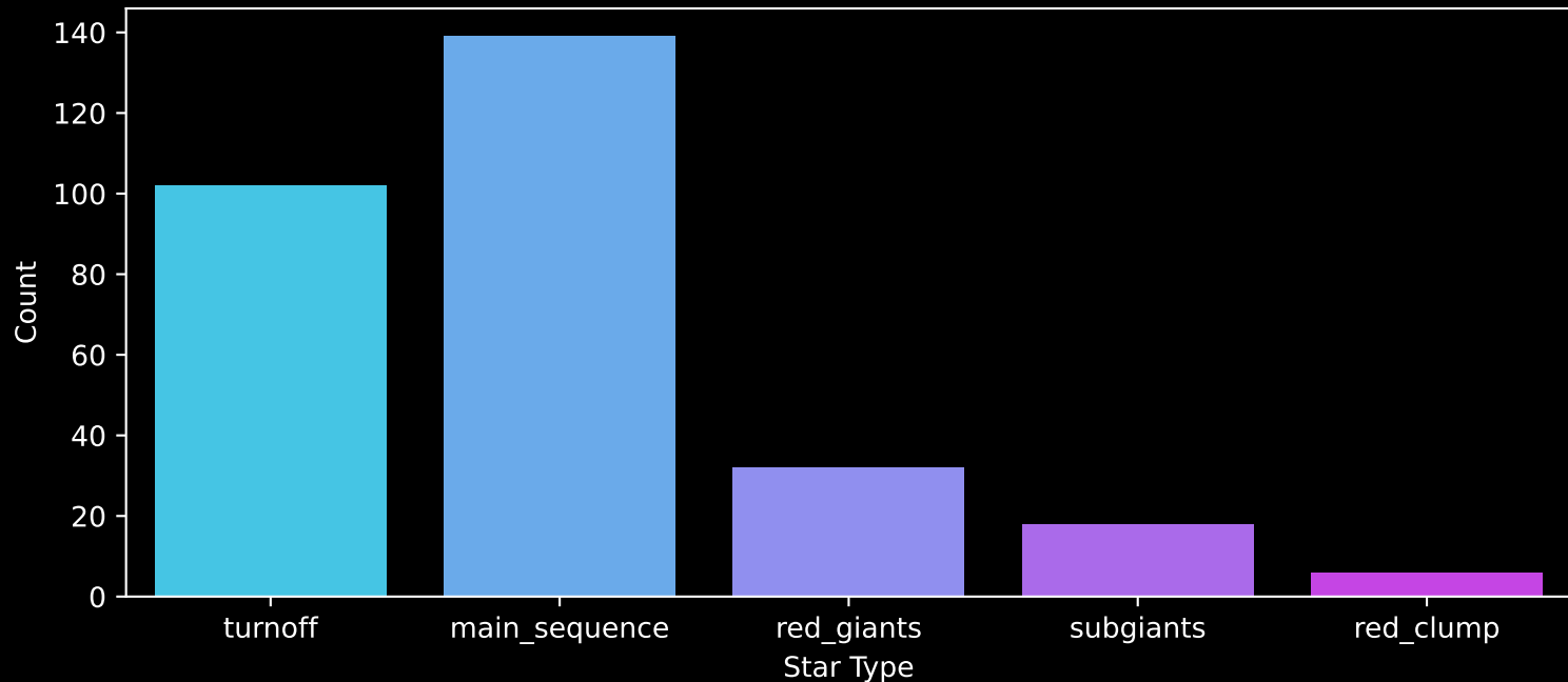
GALAH DR4 Field: [1616] Count plot of Star Type
