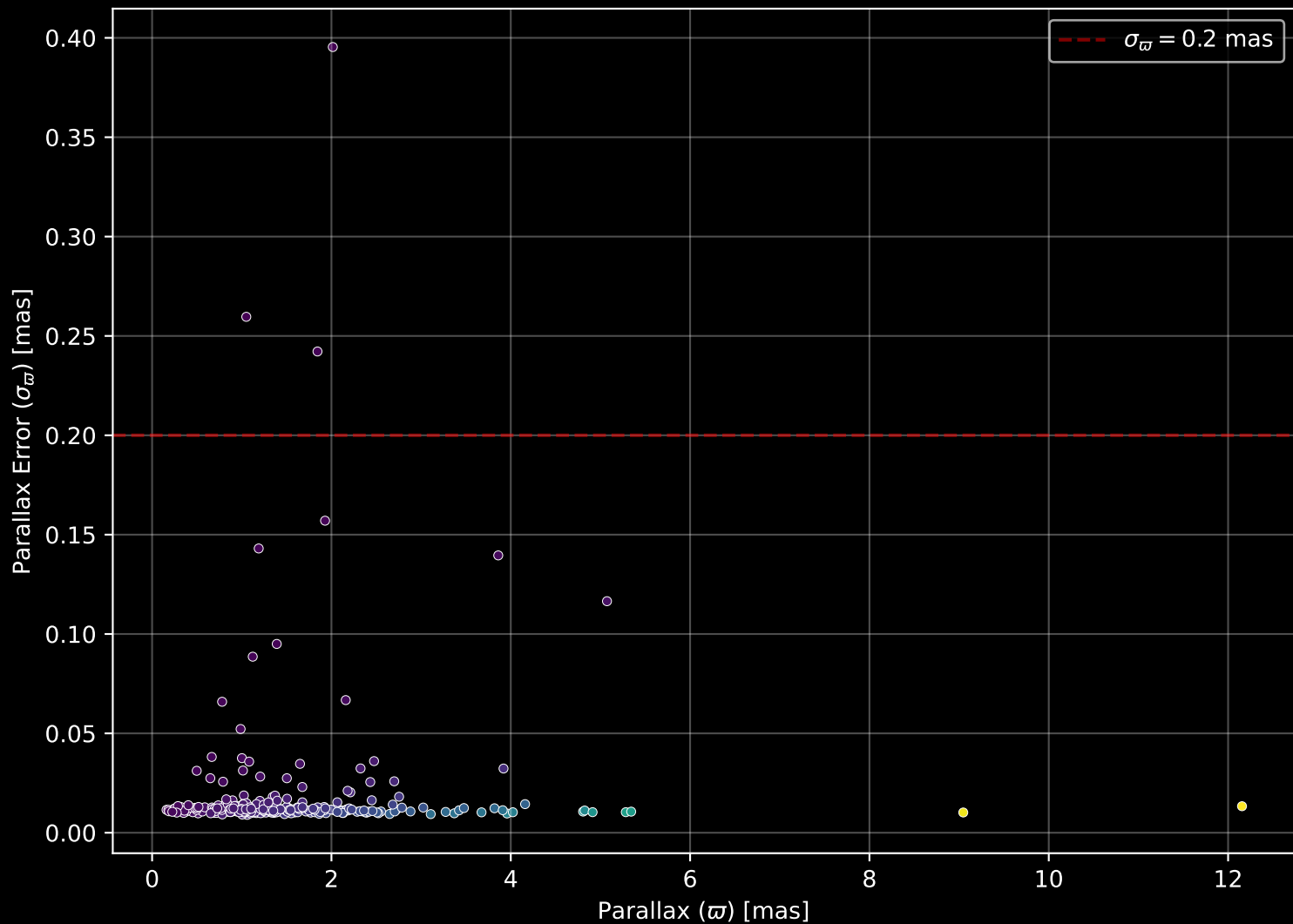
GALAH DR4 Field: [1616] Parallax Quality (n= 297)
