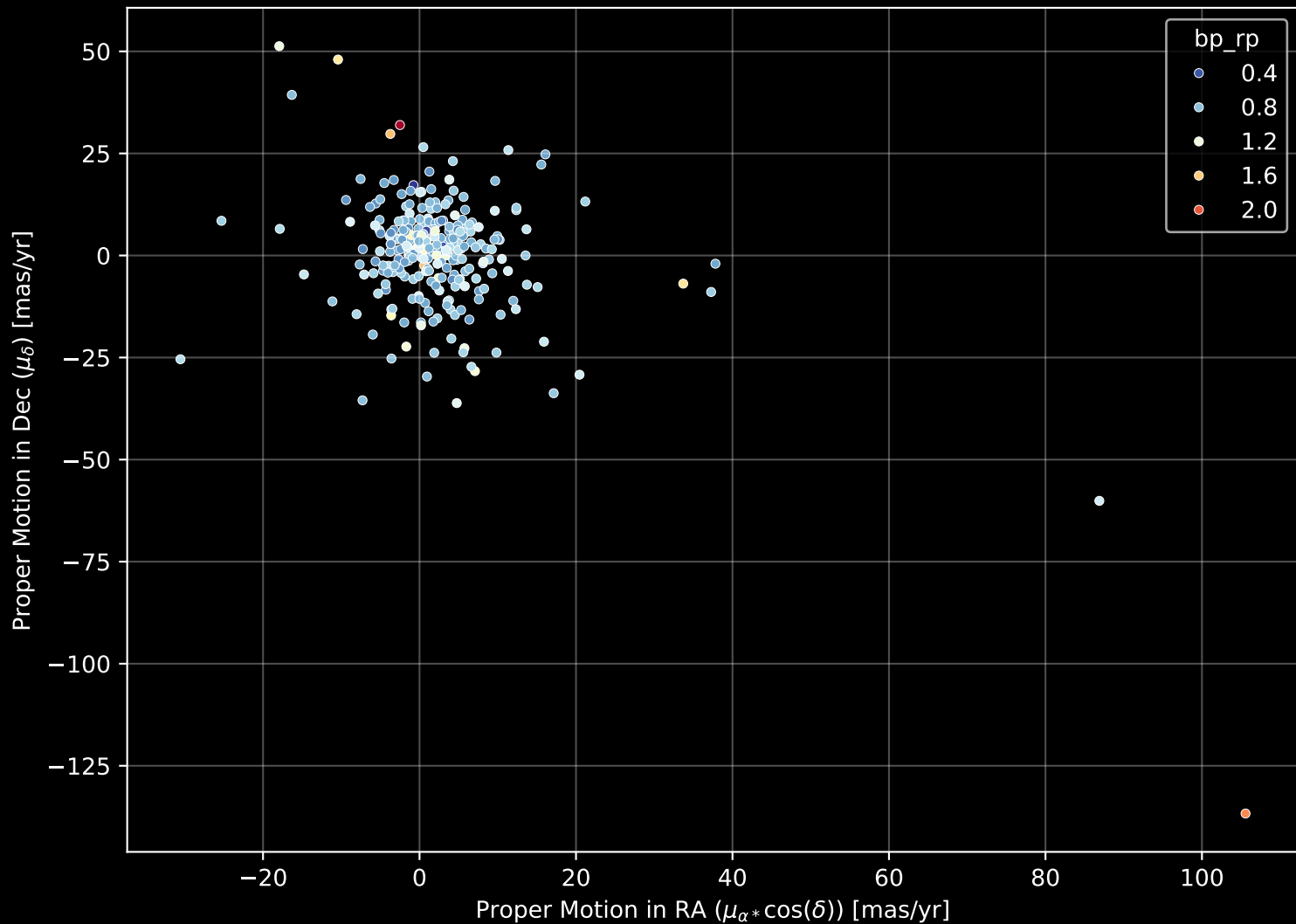
GALAH DR4 Field: [1616] Proper Motion Diagram (n= 297)
